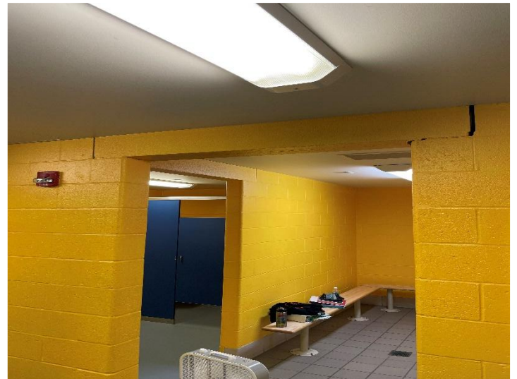
Several door lintels have pulled apart. Additional civil engineering and geotech report are anticipated.
